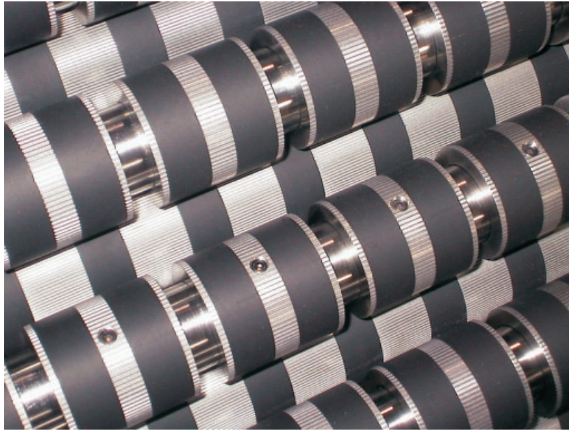
Setscrew-locking segments
